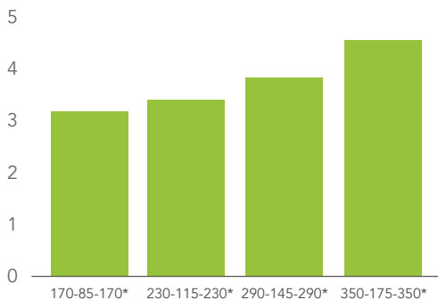
Figure 1: Effect of different fertilizer NPK application rates (N: P 2 O 5 : K 2 O = 2:1:2) on average dry bean yield of coffee arabica (Var. Catimor) grown in Buon Ma Thuot, Daklak province, Vietnam 1993-1999
